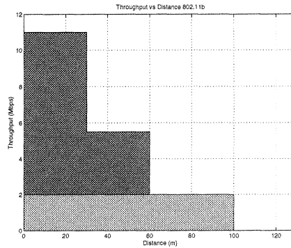
Figure 9. Distance vs Throughput in 802.11b
