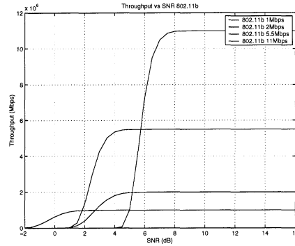
Figure 6. Throughput as a function of SNR
