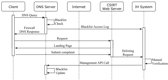
Fig. 2. Query processing in the DNS RPZ with a management interface and a logging module.
