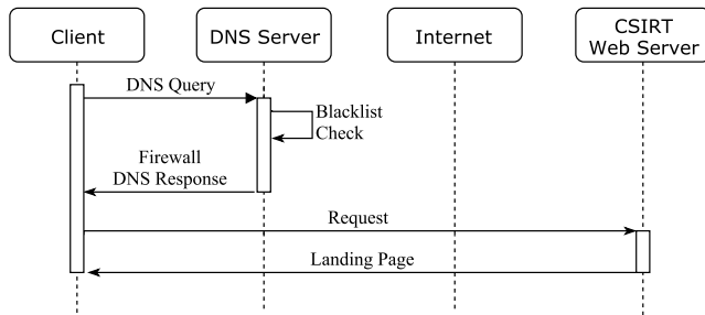
Fig. 1. Query processing in the DNS RPZ
